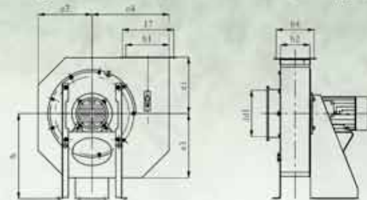
Wentylator WP-1000
