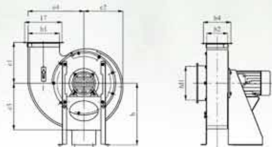
Wentylator WP-500
